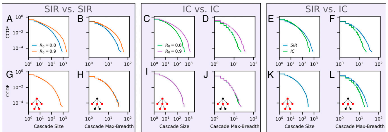
Fig. 3. (A–F) Structural statistics of datasets of cascades simulated using the SIR and IC models. (A and B) Size and maximum breadth of SIR cascades with two different values of the infectivity parameter R_0 . (C and D) Size and maximum breadth of IC cascades with two different values of R_0 . (E and F) Size and maximum breadth of SIR vs. IC cascades with the same choice of R_0 = 0.8 . (G–L) The same analyses as the plots directly above, carried out for two subsampled datasets with matched size distributions. Controlling for size collapses statistical differences in structural properties when simulations come from the same underlying model (IC or SIR), even for different choices of infectivity R_0 . The collapse does not happen if the underlying models are different. Insets again depict each statistic on a simple cascade. Only size and breadth are shown here due to space constraints; the collapses of the remaining statistical quantities are shown in SI Appendix, Figs. S14, S18, and S22 .
